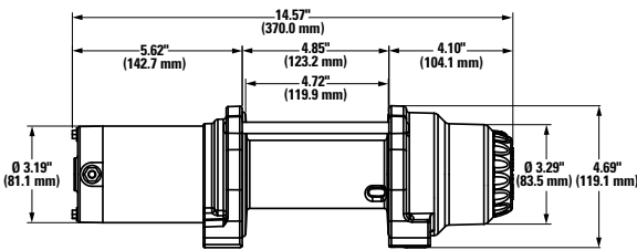
Winch dimensions: 14.57" L x 4.53" D. x 4.69" H. (370mm L. x 115mm D. x 119mm H.)
