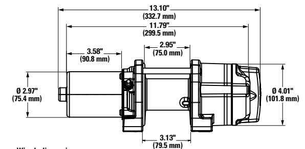
Winch dimensions: 13.1" L x 4.53" D x 4.69" H. (331.6mm L x 115mm D x 119mm H.)
