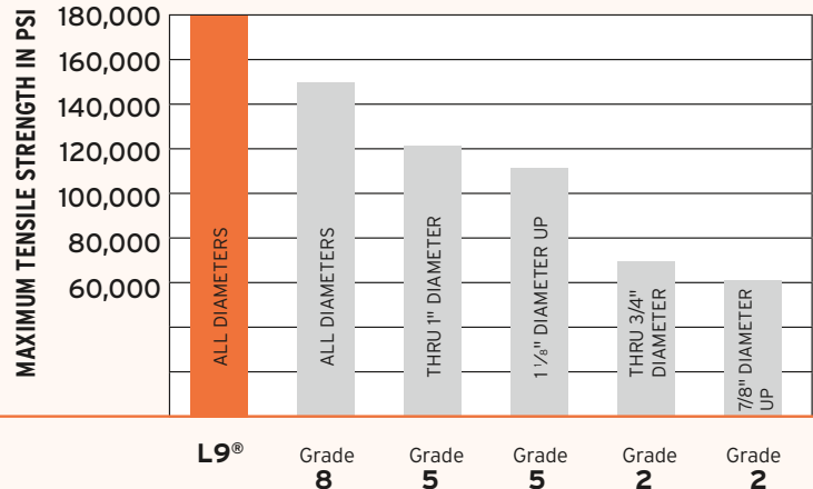
COMPARATIVE STRENGTHS SAE GRADES 2, 5, 8 AND L9® BOLTS
